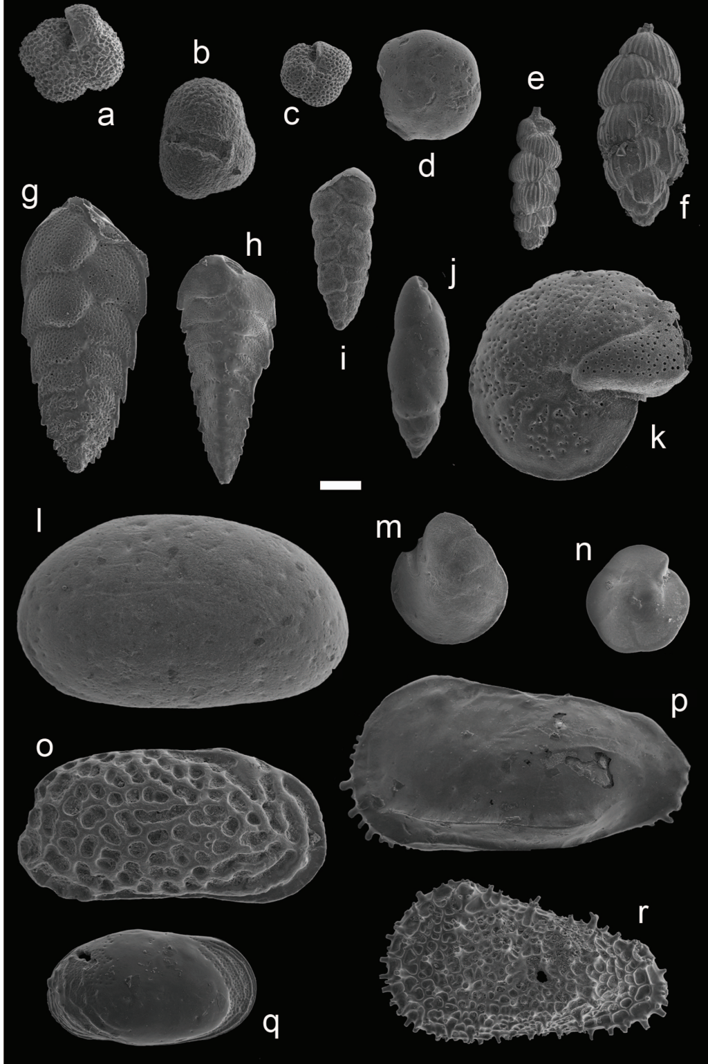
Appendix 2. Selected species of foraminifera and ostracods recovered from the T-191 borehole cuttings. a. Neogloboquadrina dutertrei , sample 110 m; b. Sphaeroidinellopsis seminulina , sample 220 m; c. Neogloboquadrina acostaensis dx, sample 220 m; d. Ammonia sp., sample 90 m; e. Uvigerina cf. U. pygmaea , sample 150 m; f. Uvigerina bononiensis , sample 150 m; g. Bolivina alata , sample 150 m; h. Bolivina spathulata , sample 150 m; i. Bolivina punctata , sample 150 m; j. Bulimina exilis , sample 150 m; k. Cibicidoides ungerianus , sample 190 m; l. Cyprideis agrigentina , sample 230 m; m. Cibicidoides kullenbergi , sample 190 m; n. Oridorsalis umbonatus , sample 190 m; o. Urocythereis exedata , sample 110 m; p. Ruggieria tetraptera , sample 110 m; q. Rectobuntonia subulata , sample 150 m; r. Acanthocythereis hystrix , sample 110 m. White bar corresponds to 0.1 mm.
